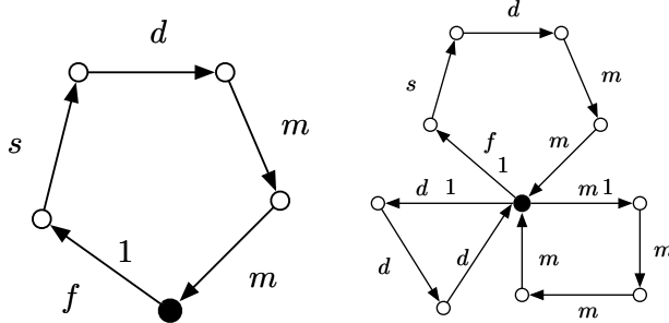
Figure 2.1. On the left is C_w , where w = \text{fsdmm} and cost of w is 1. On the right is G_{w,s} where W = \{\text{fsdmm}, \text{ddd}, \text{mmm}\} , and the cost of each word is 1. The black vertex is the special start vertex q . Edges without weight label have weight 0.
